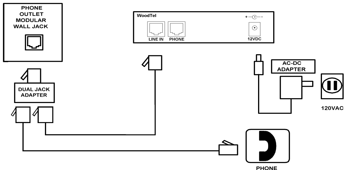
Fig. 2 Connection diagram for normal use.
