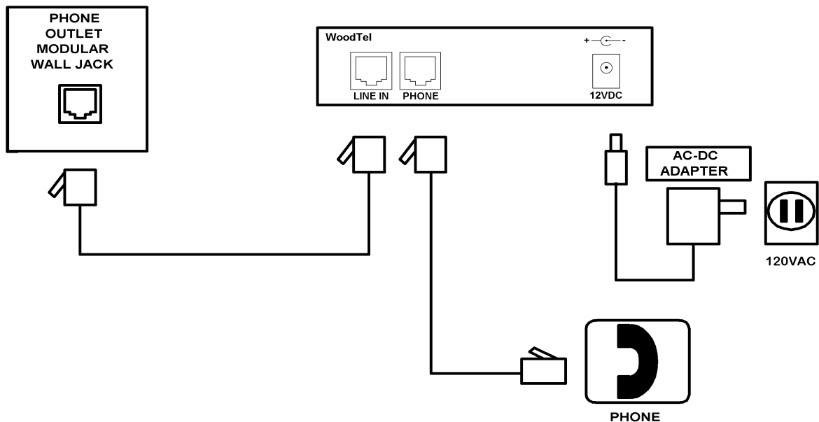
Fig. 1 Connection diagram for on-site programming
